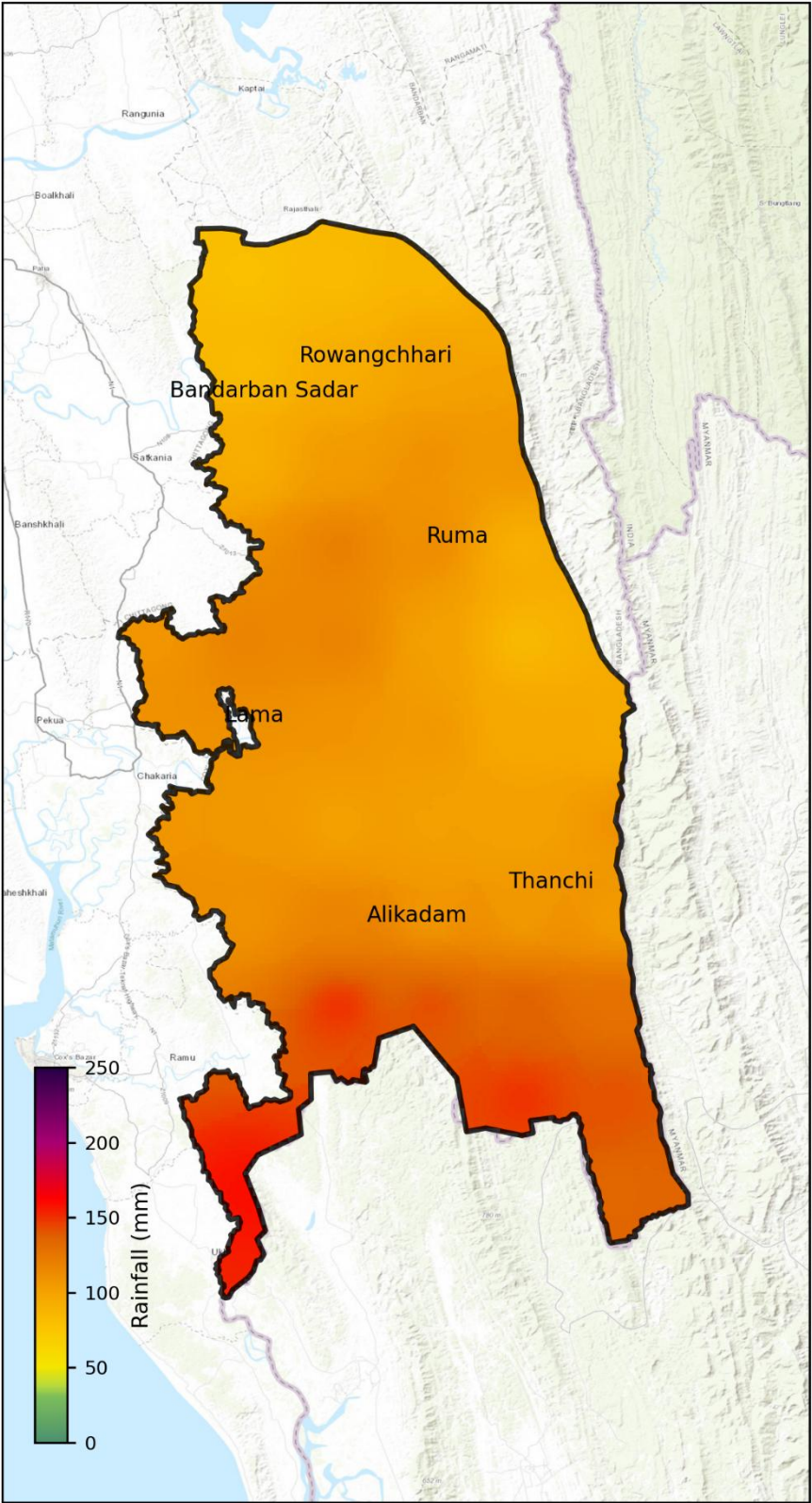
ECMWF 72 h Accumulated Rainfall Forecast over Bandarban (09-11 July 2026)
